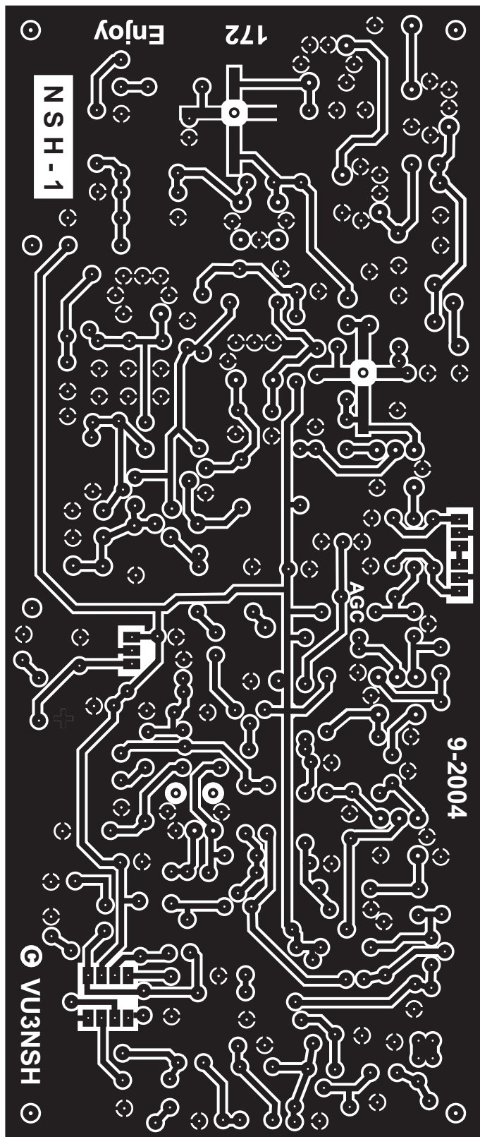
NSH-1 7MHz RECEIVER - SOLDER SIDE LAYOUT
